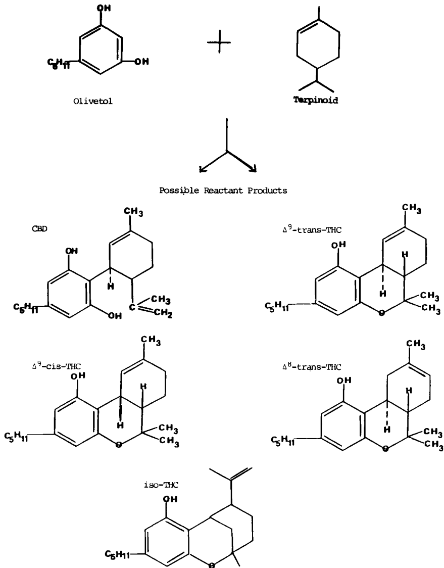
FIG. 2—Possible products of olivetol and terpinoid reaction.
