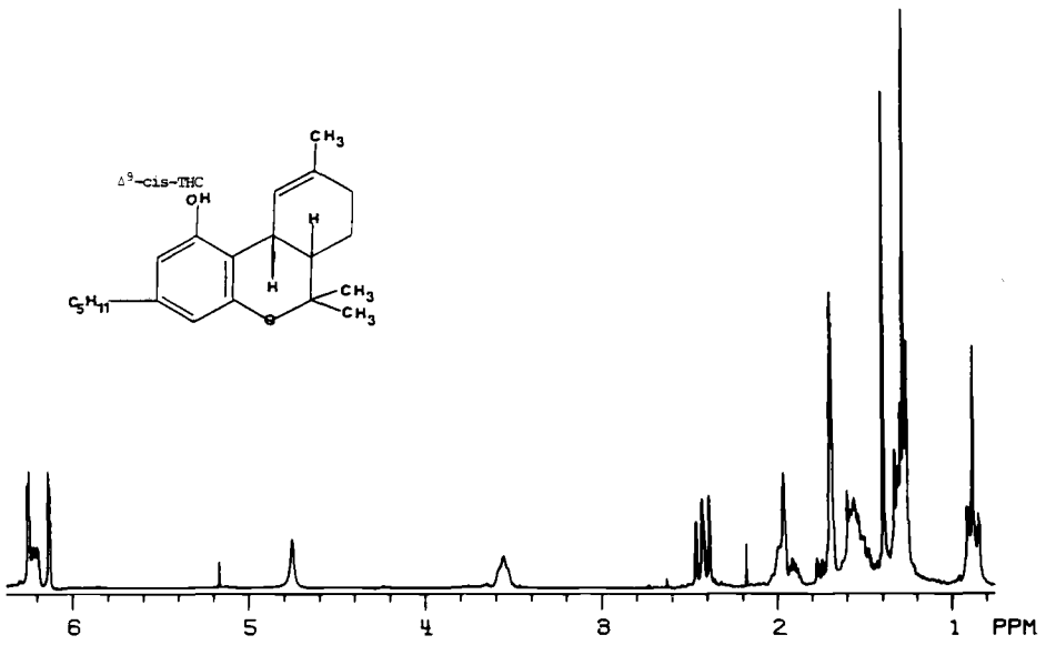
FIG. 13—NMR spectrum of \Delta^9 -cis-tetrahydrocannabinol.
