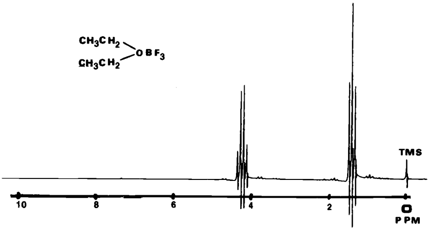
FIG. 6—NMR spectrum of boron trifluoride etherate.
