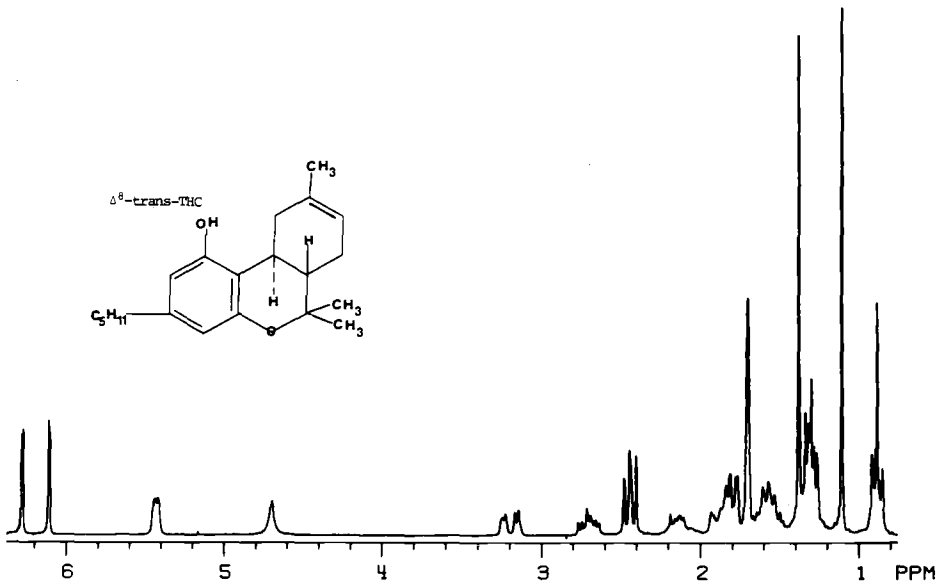
FIG. 15—NMR spectrum of \Delta^8 -trans-tetrahydrocannabinol.
