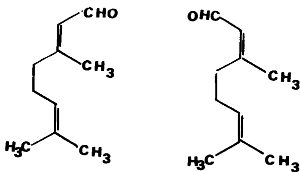
FIG. 4—Geranial (citrinal A) on left and neral (citrinal B) on right.
