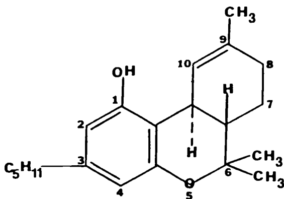
FIG. 1—Skeletal cannabinoid structure.
