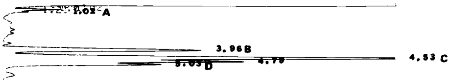
FIG. 7—GLC of Sample 2 with \Delta^8 -trans-THC added.
