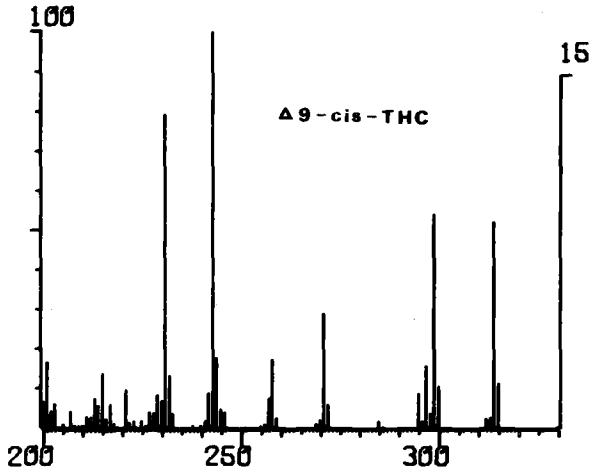
FIG. 9—Partial mass spectrum of \Delta^9 -cis-tetrahydrocannabinol.
