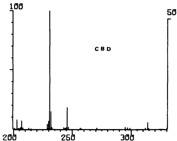
FIG. 8—Partial mass spectrum of cannabidiol.
