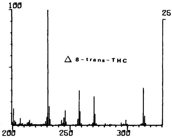
FIG. 10—Partial mass spectrum of \Delta^8 -trans-tetrahydrocannabinol.
