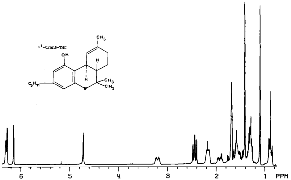
FIG. 14—NMR spectrum of \Delta^9 -trans-tetrahydrocannabinol.
