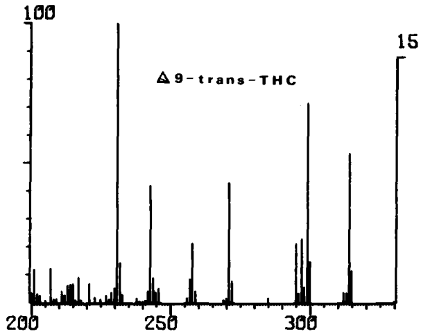
FIG. 11—Partial mass spectrum of \Delta^9 -trans-tetrahydrocannabinol.
