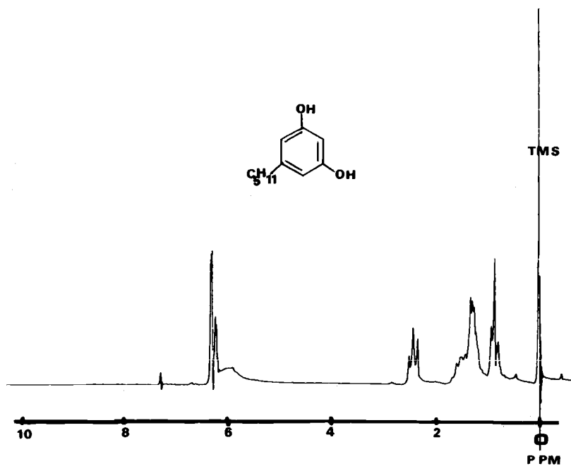
FIG. 3—NMR spectrum of olivetol.
